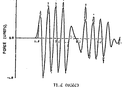
2. MHZ EXCITATION BURST (4 CYCLE)
