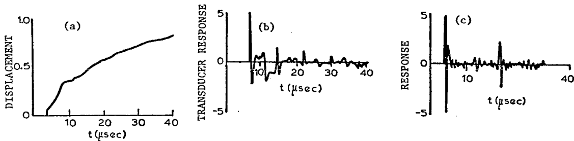
Figures 10(a) - 10(c) - Determination of a piezoelectric receiver's transfer function (a) Epicenter displacement, step-unloading source, (b) Piezoelectric transducer signal, step-unloading source, (c) Result of the deconvolution, T(t) .
