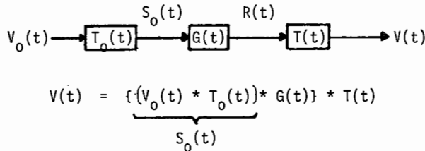
Figure 2 - A linear ultrasonic system.
