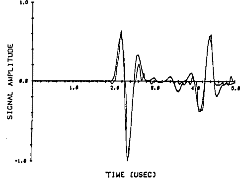
Figures 8(a) and 8(b) - Measured and predicted signals detected from two excitation functions.
