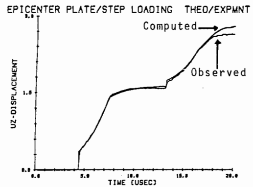
Figure 3 - Epicentral displacement: step unloading. Computed, observed.
