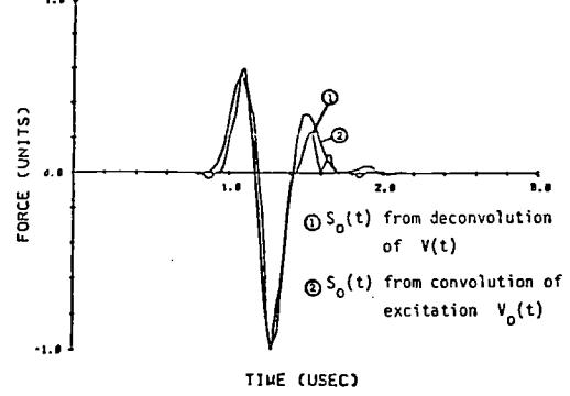
2. MHZ EXCITATION BURST (SINGLE CYCLE)
