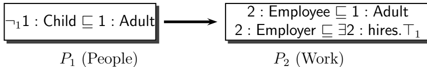
Fig. 1. Semantic Importing
