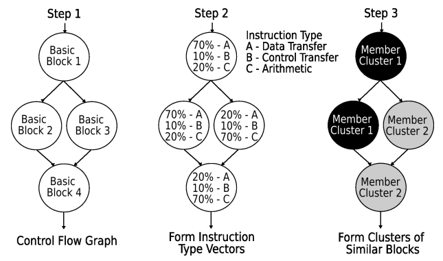
Figure 2. Clustering
