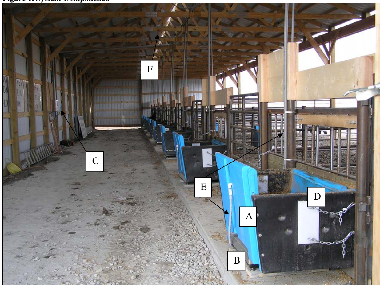
Key to labels: A=stock Miraco feed bunk, B=Rice Lake bench scale, C=Rice Lake scale indicator, D=embedded RF antenna, E=shielded cable runs, F=RF reader
