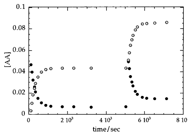
Figure 1. Kinetic trace obtained by NMR spectroscopy for the isomerization of 3-methyl-2-buten-1-ol (decreasing with time) to 2-methyl-3-buten-2-ol (increasing with time). [\text{MTO}] = 25 \text{ mM} , [\text{AA}] = \text{allyl alcohol} = 50 \text{ mM} . The second stage of the reaction indicates a second addition of 3-methyl-2-buten-1-ol.
