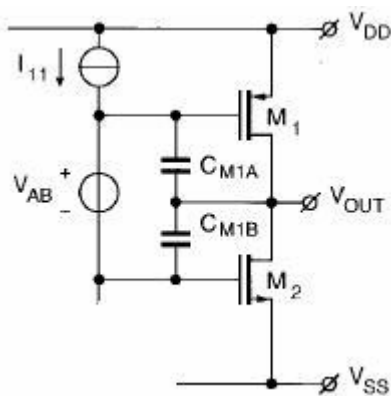
Figure 2-4. Class-AB Output Stage (modified) [7]
