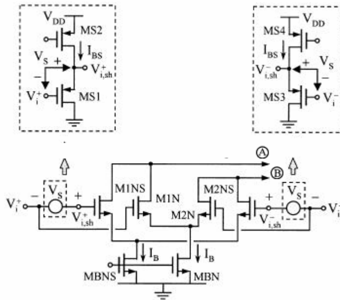
Figure 2-8. Dual n-ch Input Pair with Level Shift (modified) [9]
