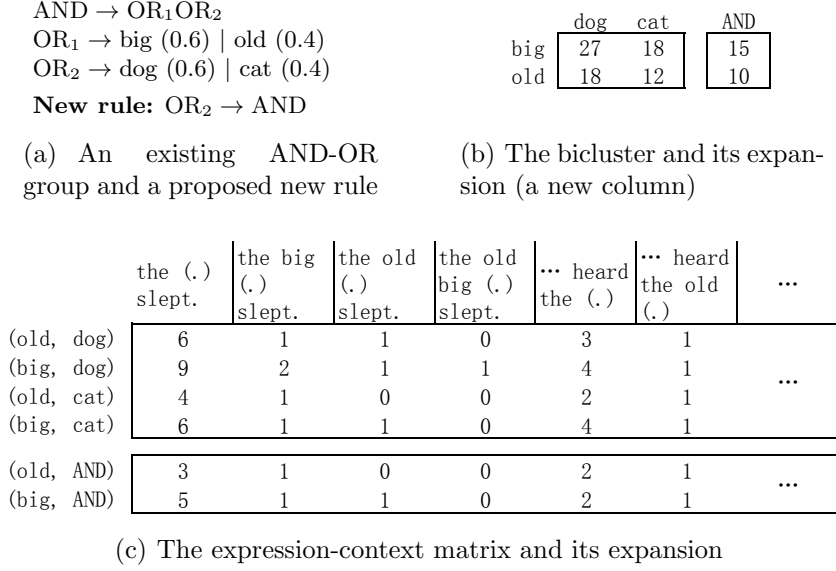
Figure 3.2 An example of adding a new rule that attaches a new AND under an existing OR. Here the new AND is attached under one of its own OR symbols, forming a self-recursion.
