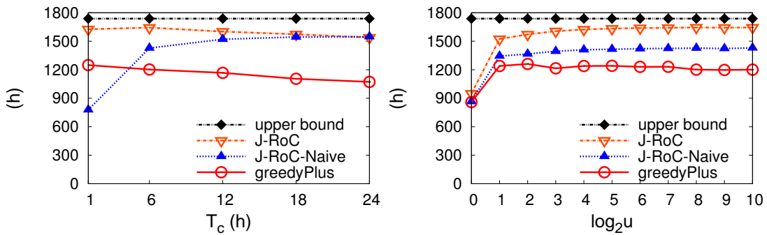
(a) Network lifetime with varying T_c .
