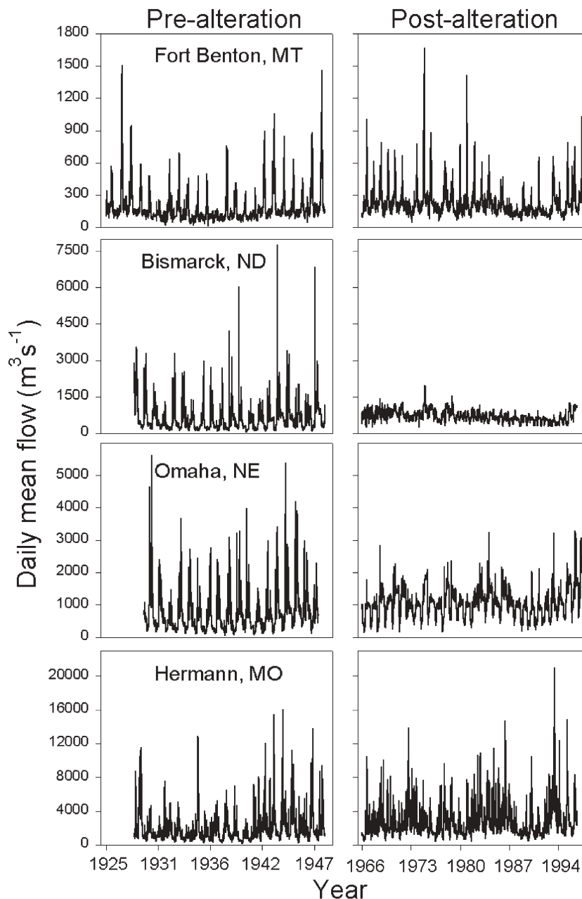
Figure 2. Daily mean flows during the pre-alteration (1925–1948) and post-alteration (1967–1996) periods at four representative gauges along the Missouri River.
