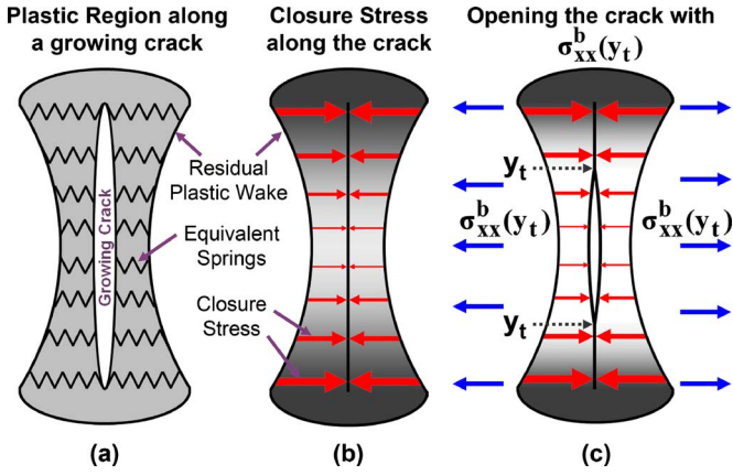
FIG. 2. (Color online) Crack closure model showing (a) the plastic region as the crack advances, (b) closure stresses along a crack due to the compression of the plastic region, and (c) opening the crack with an applied load to track the closure transition points, y_t , as a function of the applied load.
