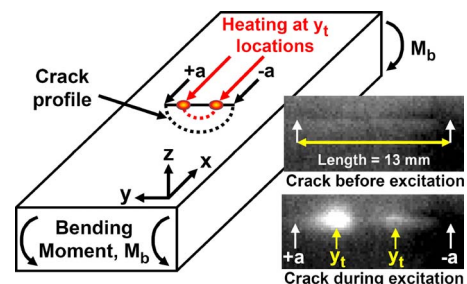
FIG. 1. (Color online) Schematic of a crack in a test bar. The right side shows the IR images of a stationary crack (top) and the IR heating when the crack is vibrated (bottom). Crack tips are located at \pm a .
