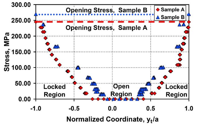
FIG. 4. (Color online) Crack opening stresses and closure stress profiles along the lengths of two cracks calculated from measures of y_i and Eq. (2) and normalized by y_i/a .
