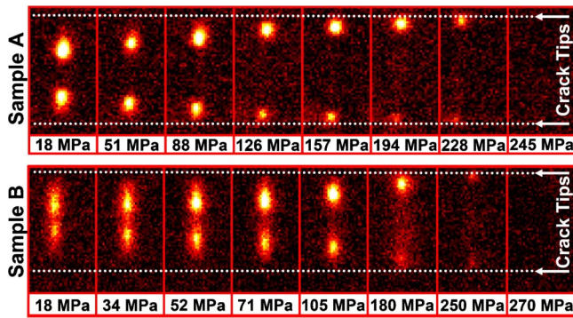
FIG. 3. (Color online) Regions of crack heating as a function of applied bending stress. The far right images show the crack opening stress or the applied stress required to fully open the crack and terminate heat generation.
