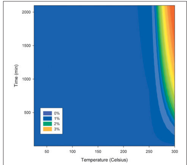
Figure 7 Contour map of Au-7at% Pt showing only the most significant time and temperature range for engineering applications such as interconnection wire. Percentages shown in the key are percent change of resistivity
