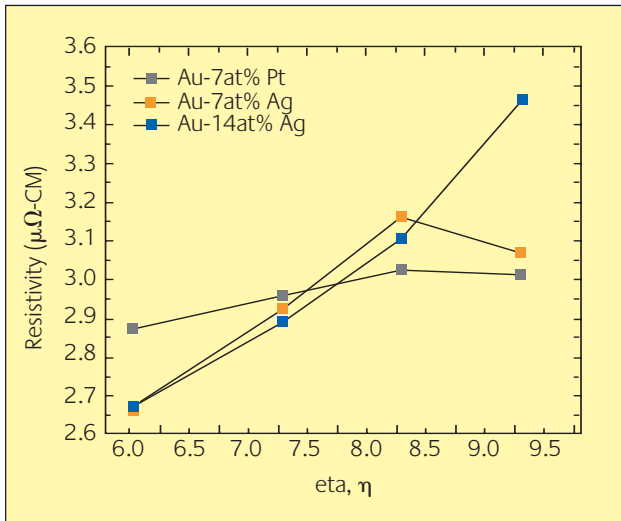
Figure 3 The relation between resistivity and deformation true strain. Note that resistivity increases with increasing true strain deformation ( \eta ). Note that the Au-7 at%Ag and Au-7 at%Pt decrease at the highest deformation level, but the Au-14 at%Ag does not
