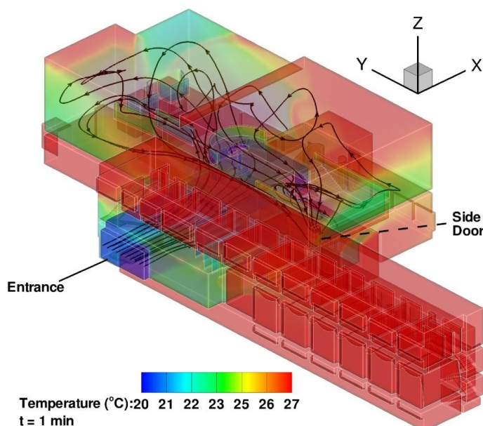
Figure 5: Internal air flow pattern at Viipuri library
