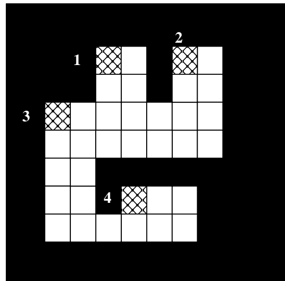
Figure 2. Example of an object with more than one chain code starting pixel, shown as cross hatched. All of the cross hatched pixels 2-4 are also a part of the chain code starting with candidate pixel 1.
