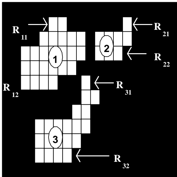
Figure 3. In the first step of the fusion process, only objects contained within the row limits ( R_{x1} and R_{x2} ) of another object are considered for fusion. Object 2, for example, is completely within the row limits of Object 1 ( R_{21} \geq R_{11} and R_{22} \leq R_{12} ) hence objects 1 and 2 are considered for fusion. Object 3 is not considered in this step.
