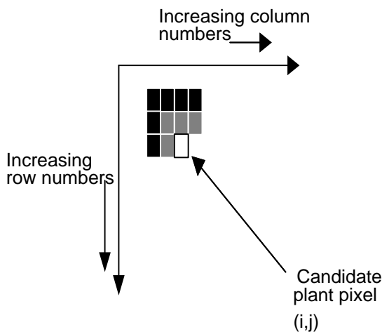
Figure 1. Chain codes were always started from the upper left corner of objects. The algorithm determined if a detected plant pixel was at a local upper left corner of an object using the criteria given by equation 1.
