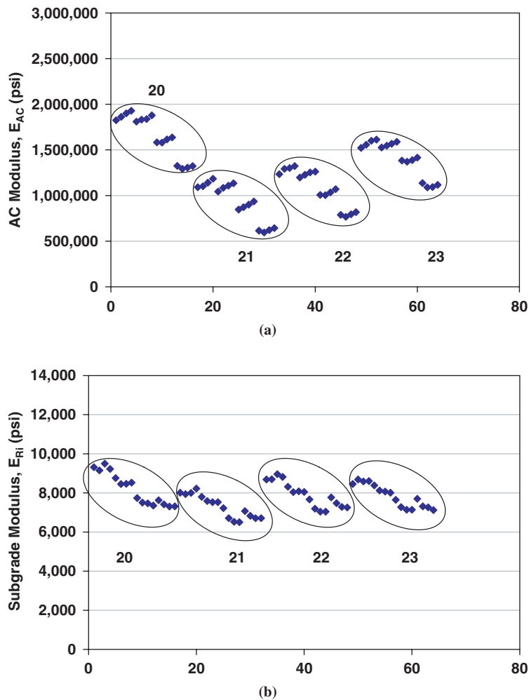
FIGURE 1 ANN-based modulus predictions for Site 2 at four FWD test points (X-axis represents number of FWD drops): (a) AC moduli and (b) subgrade moduli.
