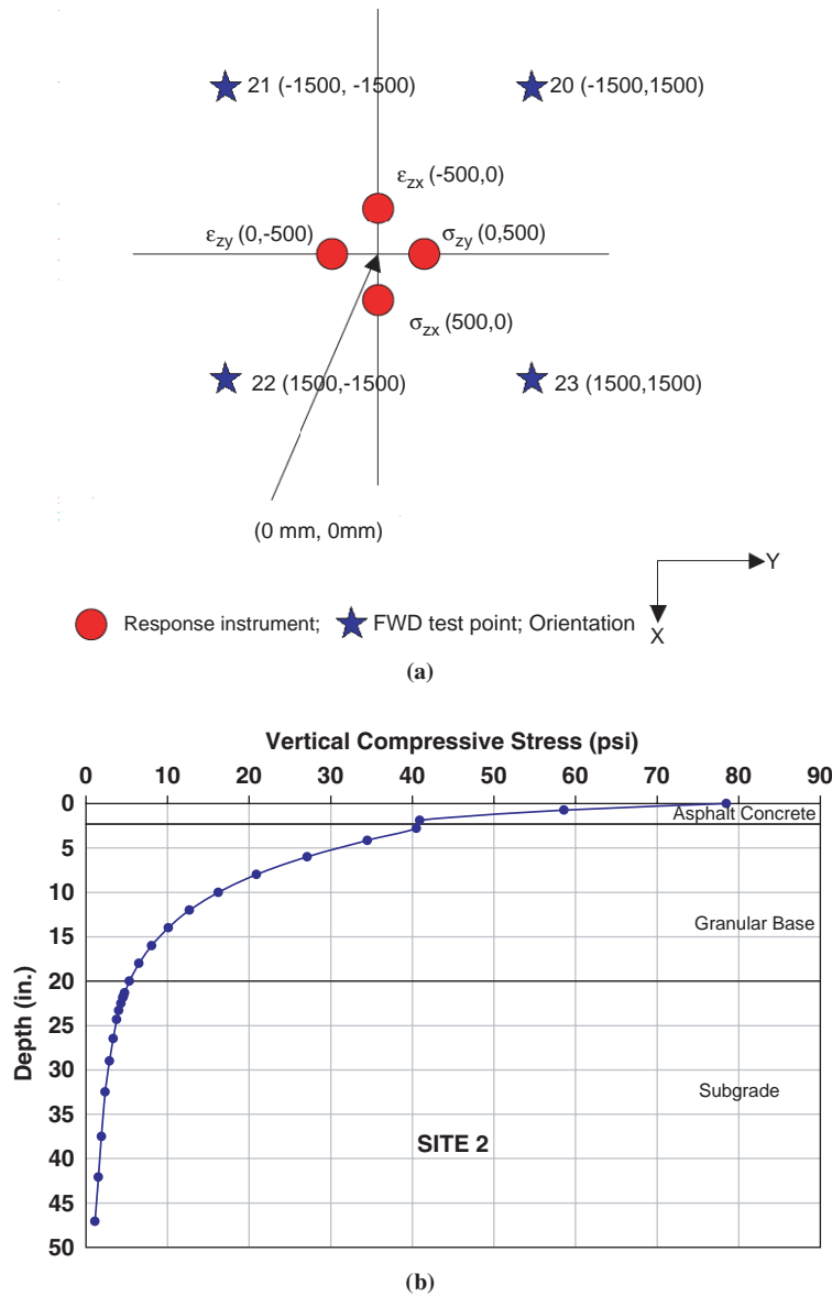
FIGURE 2 (a) Site 2 test area layout (12) and (b) Illi-Pave computed vertical compressive stress distribution for Site 2.
