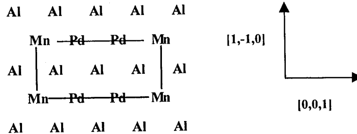
Figure 3c. 1 \times 3 domain.
