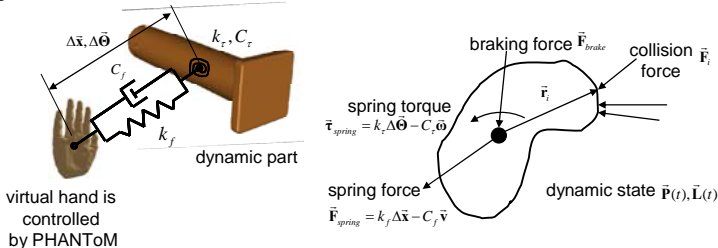
Figure 2: Physics modeling of object using VPS
