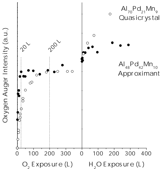
Figure 2. Oxygen uptake on the Al_{70}Pd_{21}Mn_9 quasicrystal (○) and the Al_{48}Pd_{42}Mn_{10} approximant (●) surfaces as a function of exposure to oxygen followed by exposure to H 2 O vapor. The exposure to O 2 results in the formation of a thin film of aluminum oxide which passivates the surface against further oxidation by O 2 . Subsequent exposure to H 2 O vapor results in a thickening of the oxide film followed by passivation at a higher film thickness. The rate of oxidation of the Al_{48}Pd_{42}Mn_{10} approximant during initial exposure to O 2 is roughly ten times greater than the initial rate of oxidation of the Al_{70}Pd_{21}Mn_9 quasicrystal.
