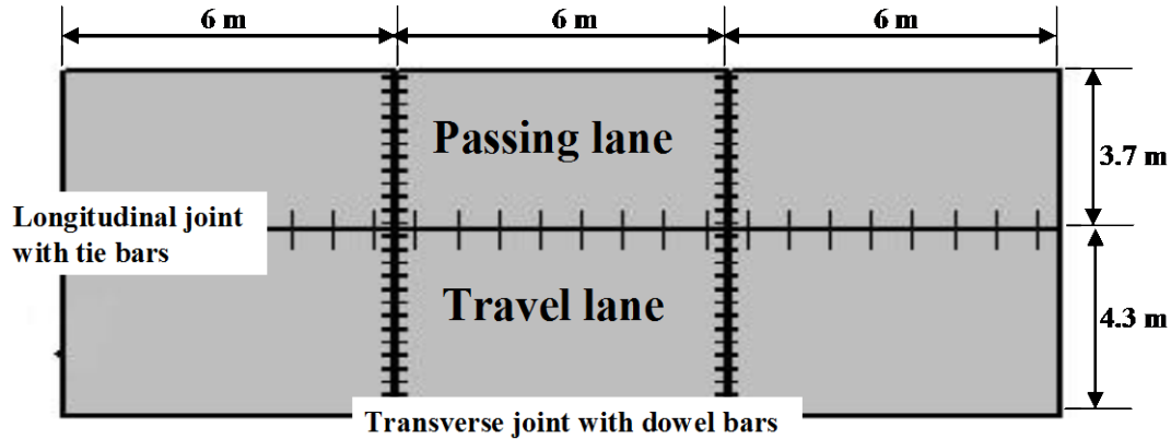
Fig. 5. PCC slab systems layout used in FE simulation
