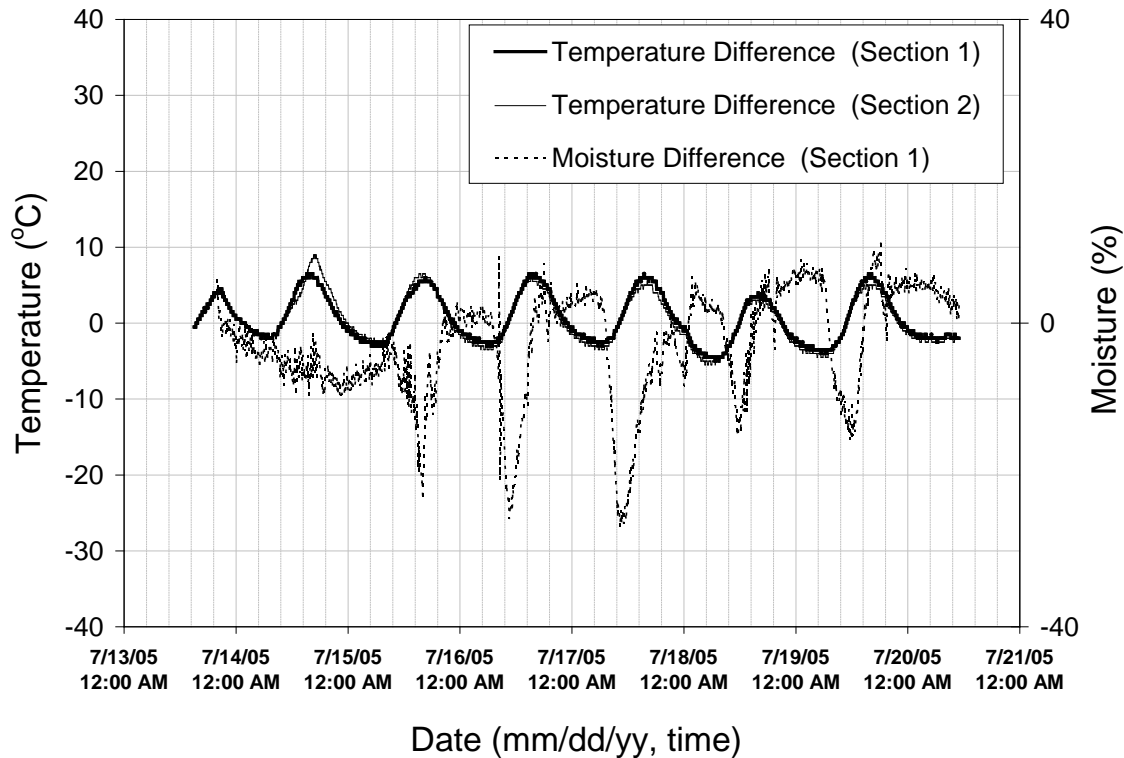
Fig. 3. Pavement temperature and moisture difference between the top and the bottom of slab with time
