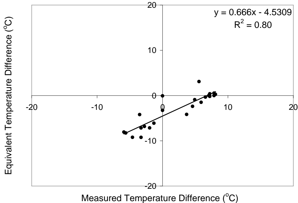
Fig. 6. Equivalent temperature difference versus measured temperature difference
