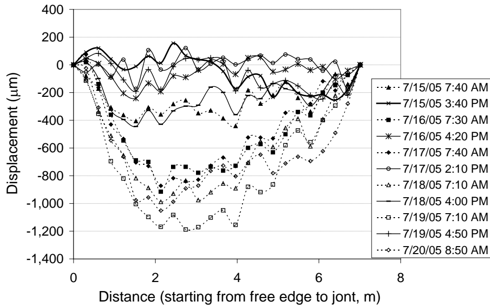
Fig. 4. Typical diagonal direction slab curvature profile (test section 1)
