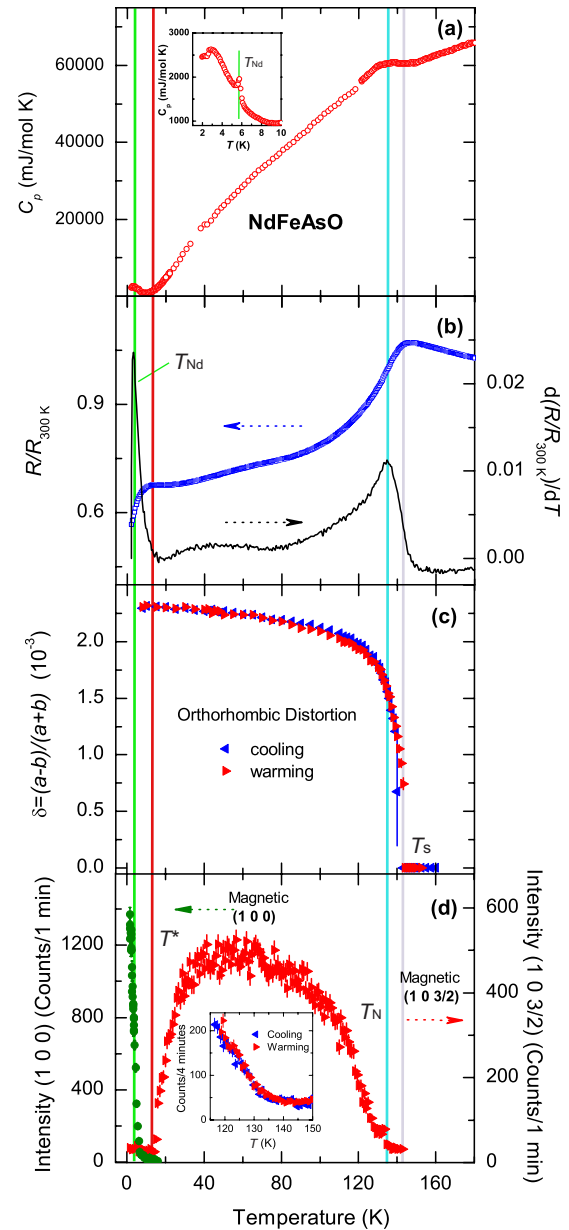
FIG. 1. (Color online) (a) Temperature dependence of the specific heat. (b) Resistivity (open symbol, left axis) and its derivative (line, right axis). (c) Orthorhombic distortion, \delta , determined by x-ray diffraction as described in the text. (d) Neutron peak intensity for the magnetic Bragg peaks at (1 0 0) (left axis) and at (1 0 3/2) (right axis). The insets show expanded scales.
