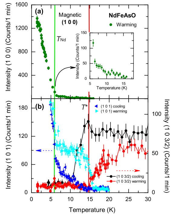
FIG. 3. (Color online) Neutron peak intensity for the magnetic Bragg peaks at (a) (1\ 0\ 0) and (b) at (1\ 0\ 1) (left axis) and (1\ 0\ 3/2) (right axis). The inset in (a) shows an expanded scale between T_{Nd} and T^* .
