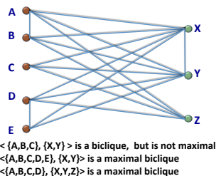
Figure 1: Maximal Bicliques
