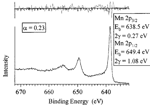
FIG. 7. Doniach-Sunjic fit to Mn 2p core-level line in \text{Al}_6\text{Mn} for the fractured surface. Solid line represent the experimental spectra, bottom dashed line is the fit, and top dashed line shows the residuals. The vertical scales for the residuals is expanded by 5 relative to the vertical scale of the experimental spectra.
