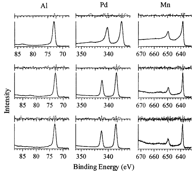
FIG. 1. Doniach-Sunjic fit to the experimental spectra for Al, Pd, and Mn. Solid lines represent the experimental spectra, bottom dashed lines are the fits, and top dashed lines shows the residuals. The vertical scales for the residuals is expanded by 5 relative to the vertical scale of the experimental spectra. The top row shows results for the pure metals. The second row shows results for the fractured fivefold surface of the quasicrystal. The bottom row shows results for the fivefold surface prepared by sputtering and annealing at 870 K.
