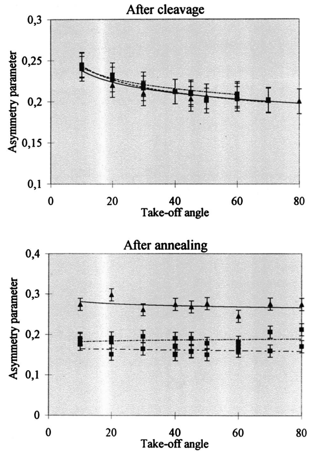
FIG. 8. Asymmetry parameter as a function of the takeoff angle, obtained from the threefold (triangles) and fivefold (squares) surface of i -Al-Pd-Mn. Amplitude of the error bars is equal to 3\sigma , where \sigma is the standard deviation.
