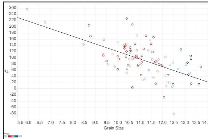
FIGURE 8. Grain size (ASTM) versus transition temperature (°F).
