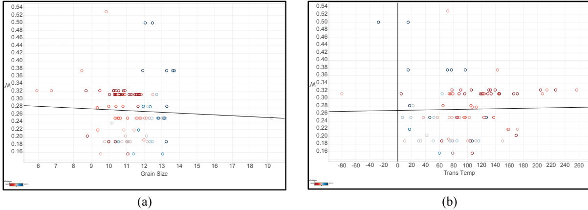
FIGURE 7. Wall thickness versus (a) grain size and (b) transition temperature.
