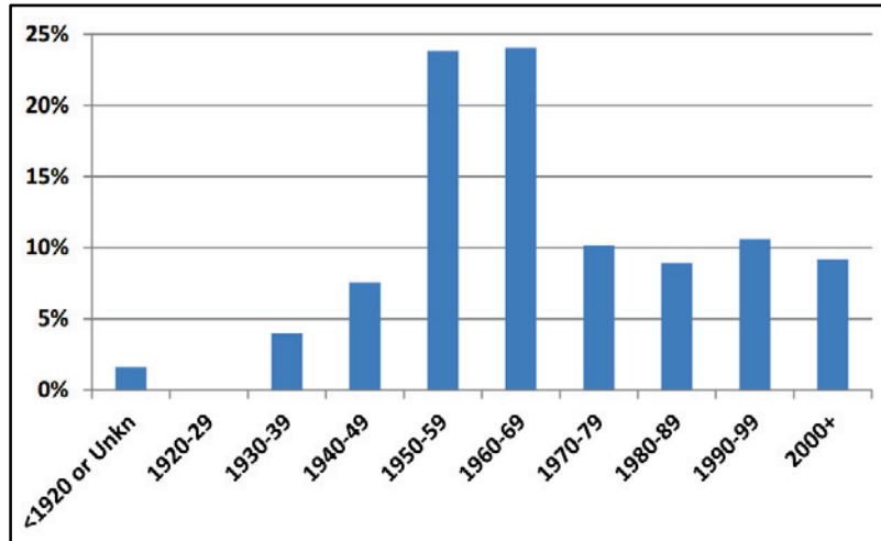
FIGURE 1. Percentage of Pipe Mileage Installed by Decade [1]
