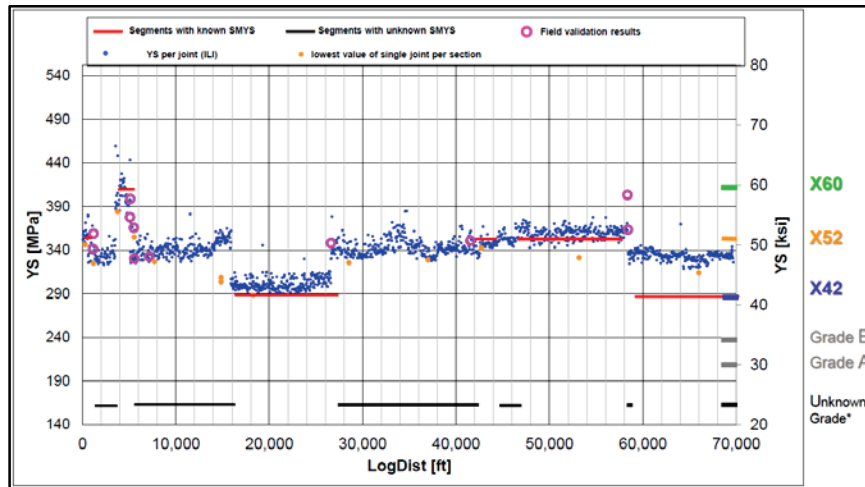
FIGURE 2. Results of the data evaluation for pipe grade determination using Rosen ILI technology. [14]
