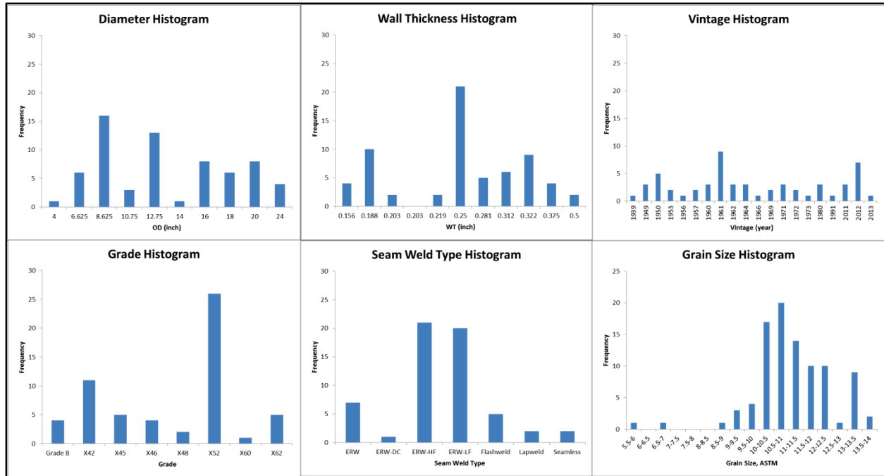
FIGURE 4. Frequency of pipe properties available from Kiefner sample data set.
