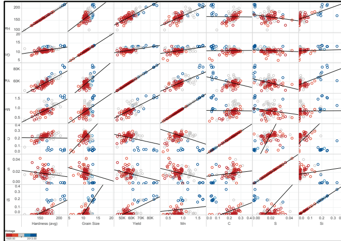
FIGURE 5. Linear regression plot comparisons for Yield, Hardness, Grain Size, %Mn, %Si, %C, %S. Vintage is indicated by the color scale, blue indicates newer vintage, red indicates older.
