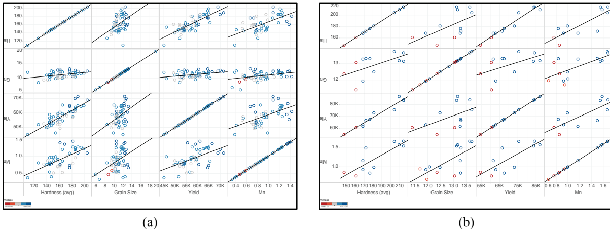
FIGURE 6. Linear regression plot comparisons for Yield Hardness, Grain Size, %Mn. (a) Pipe vintage from 1920 to 1980. (b) Pipe vintage from 1980 to 2013.
