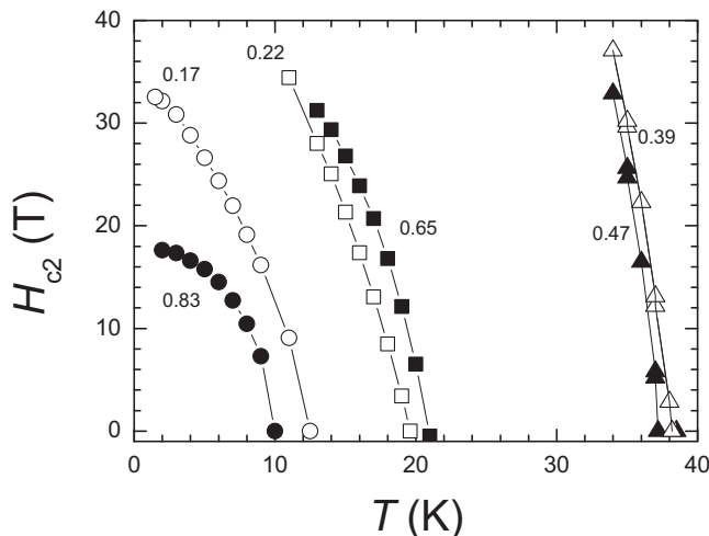
FIG. 6. Comparison of the H-T phase diagrams in parallel magnetic field H_{c2}(T) for samples of \text{Ba}_{1-x}\text{K}_x\text{Fe}_2\text{As}_2 for compositions (from left to right) with x = 0.83 (solid circles), x = 0.17 (open circles), x = 0.22 (open squares), x = 0.65 (solid squares), x = 0.39 (open triangles), and x = 0.47 (solid triangles).
