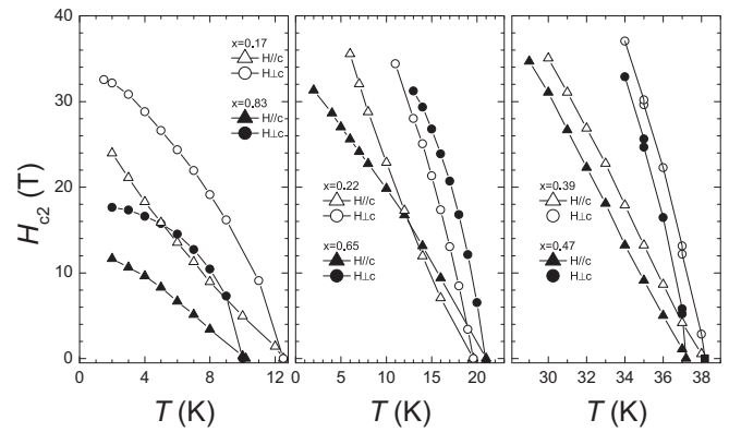
FIG. 5. Left: Comparison of the H-T phase diagrams of a 10 K pair of underdoped ( x = 0.17 ) and overdoped ( x = 0.83 ) samples. Middle: A similar comparison for a 20 K pair of underdoped ( x = 0.22 ) and overdoped ( x = 0.65 ) samples. Right: Data for samples close to optimum doping, x = 0.39 and x = 0.47 . Note the clear tendency to saturation in both overdoped compositions for the magnetic-field configuration H \parallel a .
