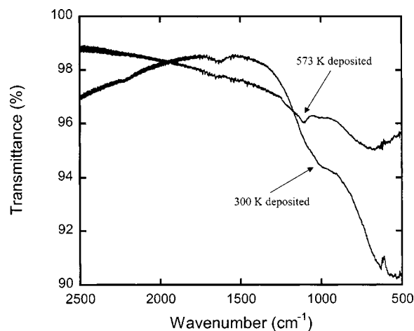
FIG. 2. FTIR spectra of the room-temperature and 573 K-deposited AlMgB 14 films.
