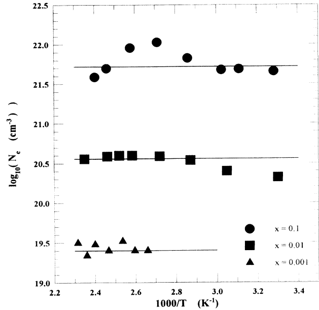
FIG. 2. The temperature dependence of \log_{10}(N_e) for glass compositions x=0.1, 0.01, and 0.001 . The points are determined by fitting each conductivity isotherm independently to Eq. (22) and the lines are determined by fitting all the conductivity isotherms simultaneously for each glass.
