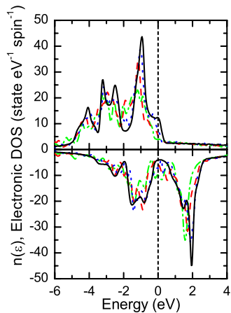
FIG. 3. (Color online) The calculated electronic density of states for \text{Fe}_{1-x}\text{Ga}_x alloys with black solid lines for x=0 (i.e., pure bcc Fe), green dashed-dotted lines for x=0.0625 , red dashed lines for x=0.125 , and blue dotted line for x=0.1875 . The positive side is for the majority spin channel, while the negative side is for the minority spin channel. Zero energy is the position of the Fermi level.
