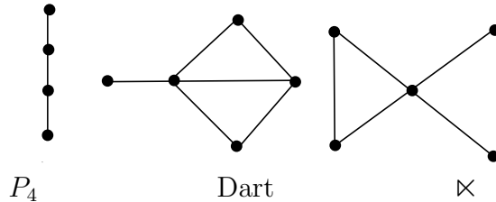
Figure 1: Some forbidden induced subgraphs for \text{mr}(\mathcal{S}_G^{\mathbb{R}}) \leq 2
