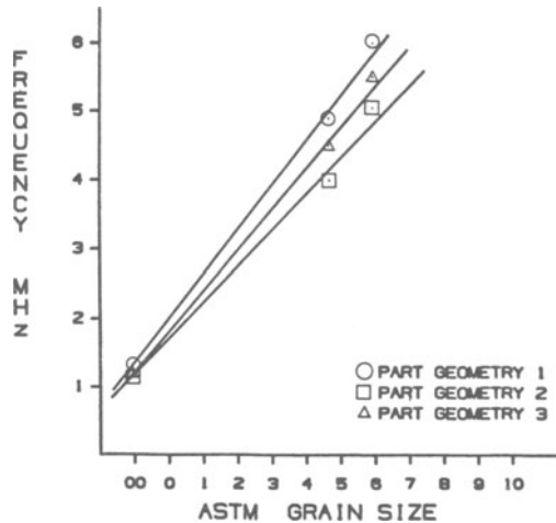
Fig. 9. Cutoff frequency vs grain size.
