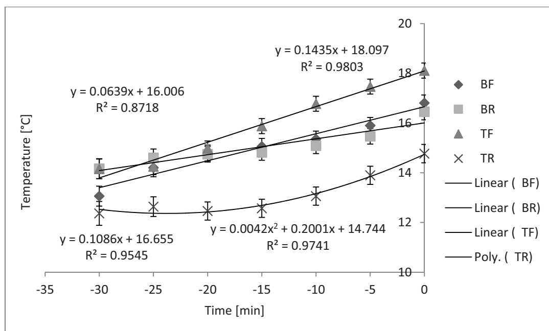
Figure 6. Compartment × time effect on internal trailer temperature while loading during mild weather ( n = 21 ). Slopes of BF, BR and TR did not differ over time. Slope of TF was linear over time while loading in mild weather ( P = 0.02 , \text{SEb} = 0.14 ).
