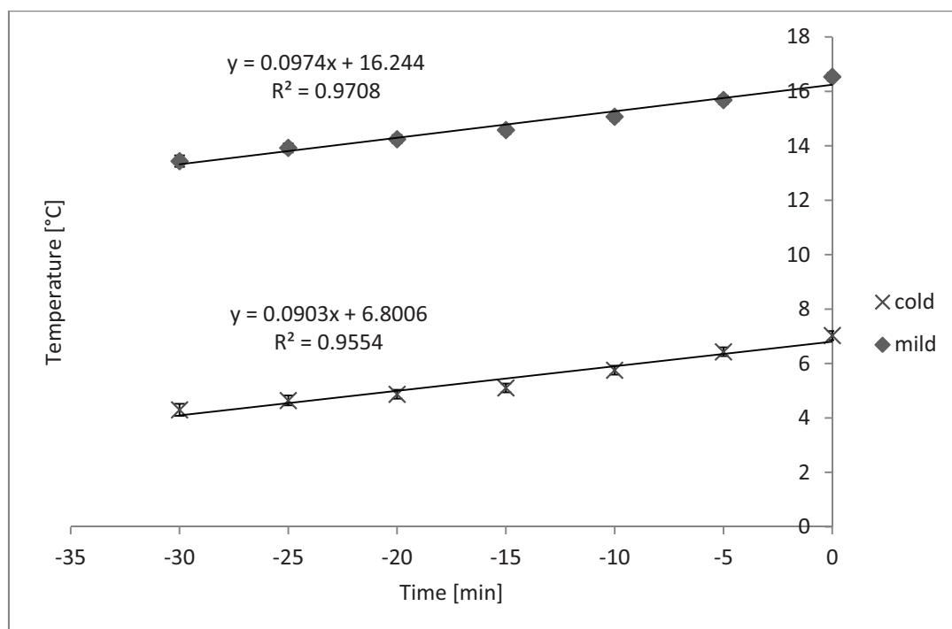
Figure 1. Overall linear time effect on average internal trailer temperature while loading during cold and mild weather ( P < 0.01 and P < 0.01 , respectively). Cold SEb = 0.06, n = 33 trailers; Mild SEb = 0.10, n = 21 trailers. Although slopes differed from zero, they did not differ between cold and mild seasons/temperatures ( P = 0.56 ).
