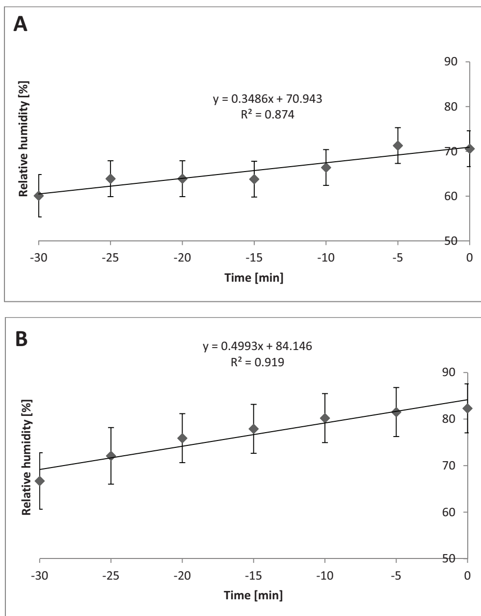
Figure 8. Relative humidity in cold weather ( n = 33 trailers) in different compartments of trailer when different levels of bedding are used. (A) Linear change in relative humidity in top front compartment while using 0.6 m 3 bedding during cold ( P = 0.03 , SEb = 0.54). (B) Linear change in relative humidity in bottom front compartment when using 1.2 m 3 bedding during cold ( P = 0.02 , SEb = 0.70). (C) Linear change in relative humidity in top front compartment when using 1.2 m 3 bedding during cold ( P = 0.01 , SEb = 0.84).
