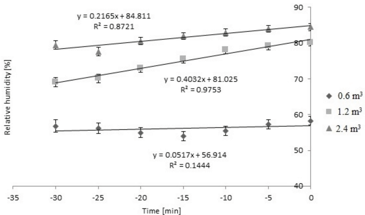
Figure 3. Bedding \times time effect on relative humidity while loading during cold weather ( P < 0.01 ). Three levels (0.6 m 3 , 1.2 m 3 , and 2.4 m 3 ) of bedding were used. Slope was 0 when 0.6 m 3 of bedding were used. Slopes differed from 0 when 1.2 m 3 , and 2.4 m 3 of bedding were used ( P < 0.05 ). 1.2 m 3 SEb = 0.03, n = 14 trailers; 2.4 m 3 SEb = 0.06, n = 12 trailers. Slopes of 1.2 m 3 and 2.4 m 3 did not differ from each other ( P > 0.05 ).
