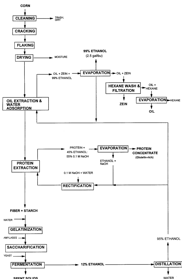
Figure 1. The original Sequential Extraction Process for corn.
