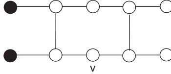
Figure 12: A graph G having Z(G - v) > Z(G)
