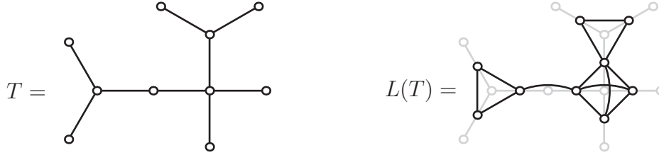
Figure 7: A tree T and its line graph L(T)
