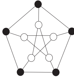
Figure 9: Zero forcing set for the Petersen graph
