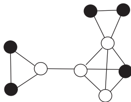
Figure 8: A zero forcing set for L(T)
