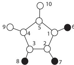
Figure 11: Zero forcing set for the corona C_5 \circ K_1
