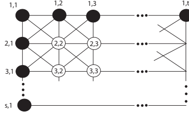
Figure 5: Zero forcing set for P_s \boxtimes P_t
