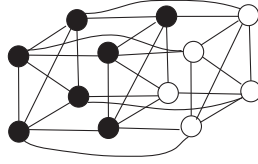
Figure 3: Zero forcing set for K_4 \square K_3
