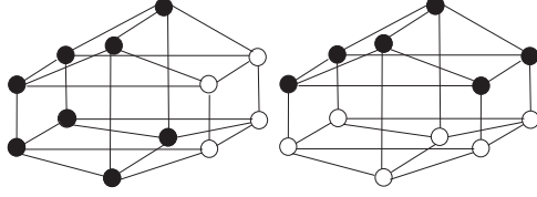
Figure 2: Two types of zero forcing sets shown on K_3 \square C_4
