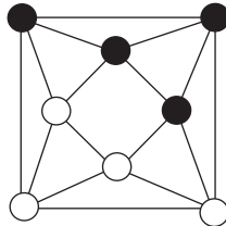
Figure 10: Zero forcing set for the 4-antiprism
