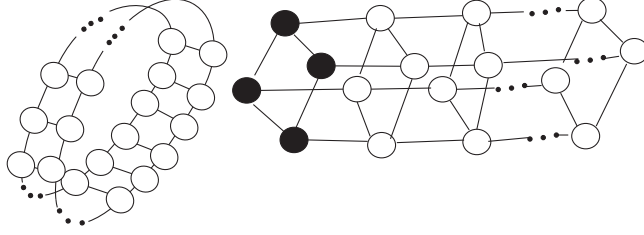
Figure 1: C_s \square P_2 and C_4 \square P_t
