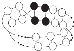
Figure 6: Zero forcing set for Möbius ladder
