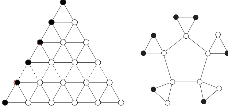
Figure 4: Zero forcing sets for supertriangle T_n and corona C_5 \circ K_2
