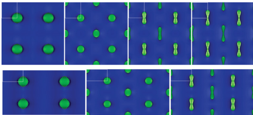
FIG. 5. (Color online) Simulated steady-state structures under the constraint of \alpha = 45^\circ (upper sequence) with \lambda values of 33.9, 101.8, 118.8, and 135.8 and \alpha = 30 \pm 1^\circ (lower sequence) with \lambda values of 32.2, 96.7, and 129.0. These simulations correspond to specific points plotted in Fig. 3. The white boxes in the top left corner of the images are the actual simulation cells.
