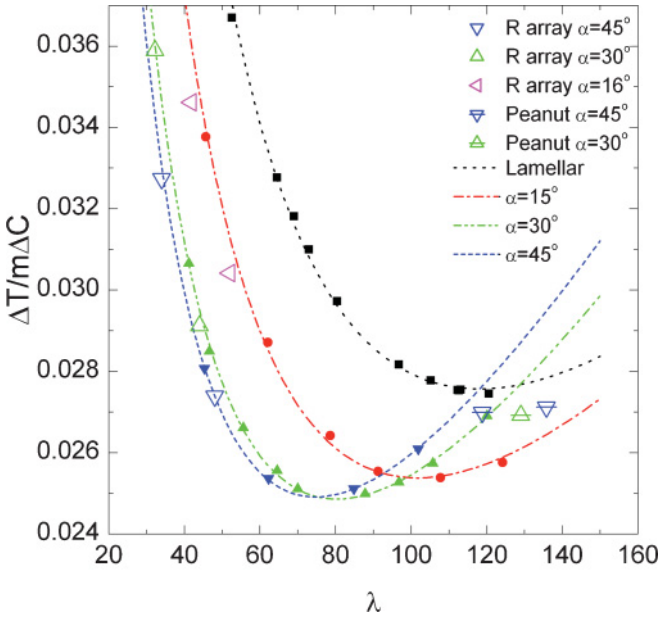
FIG. 6. (Color online) A comparison of other morphologies (empty symbols), including a rectangular array of circular rods (R array) and rods with peanut cross sections (Peanut) with a triangular array of circular rods (filled triangular and circular symbols) and lamellae (filled square symbols). The curves are JH fits to circular rods and lamellae data, which are shown in Fig. 4.
