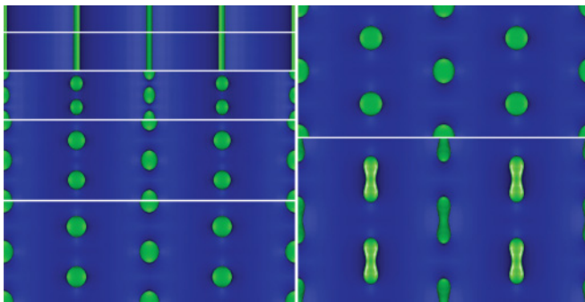
FIG. 7. (Color online) Effect of \delta on steady-state microstructures, where the width ( w = 112 ) of the simulation cell is kept constant. The starting \lambda , \delta/\lambda , and \alpha values are as follows: (a) 112.64, 0.11, and 6.12, (b) 113.14, 0.14, and 8.13, (c) 113.77, 0.18, and 10.12, (d) 116.48, 0.27, and 15.95, (e) 118.93, 0.34, and 19.65, (f) 123.48, 0.42, and 24.90, and (g) 129.00, 0.50, and 29.74.
