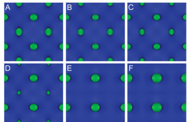
FIG. 8. (Color online) Evolution dynamics for the triangular- to rectangular-rod array transition for \alpha = 45^\circ , where the rectangular-rod array emerges after some transient time. The sequence of structures shows that the decrease in undercooling is associated with an increase in spacing that arises from the disappearance of alternating rods.
