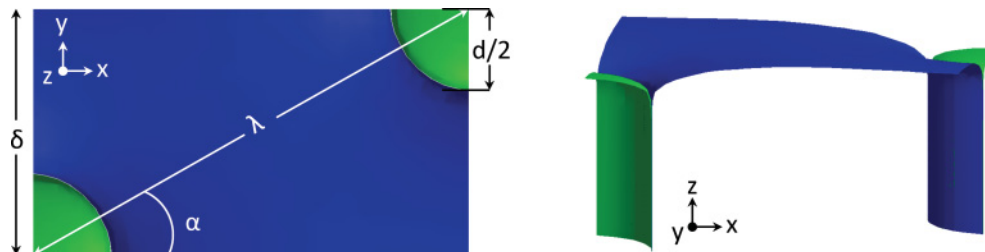
FIG. 1. (Color online) Top and 3D views of the starting simulation cell that contains two quarters of rods located in two diagonal corners. z is the growth direction.
