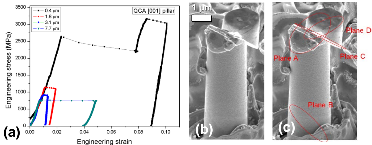
Fig. 2 (a) Representative engineering stress-strain data of \text{YCd}_6 QCA micropillars with four different diameters. We tested the total 20 micropillars (See Fig. 7); (b) Post-deformation SEM image of \text{YCd}_6 QCA micropillar after uni-axial compression; (c) shear localization traces of \text{YCd}_6 QCA micropillar. Note that shear localization occurs on four different \{1\ 0\ 1\} planes (A, B, C and D)
