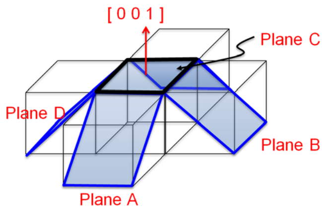
Fig. 3 Schematic diagram of \{1\ 0\ 1\} planes of \text{YCd}_6 QCA. Plane A, B, C and D correspond to those in Fig. 2(c).
