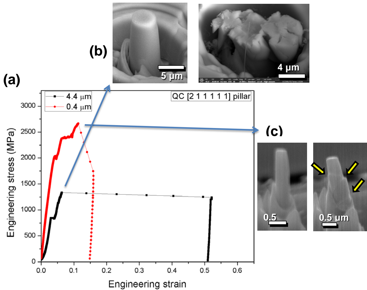
Fig. 6 (a) Representative engineering stress-strain data of i-YCd QC micropillars; (b) SEM images of a 4.4 μm diameter pillar before and after compression test; (c) SEM images of 0.4 μm diameter pillar before and after compression test
