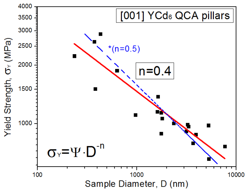
Fig. 7 A plot of yield strength of [0 0 1] YCd 6 QCA micropillars as a function of sample diameter. Blue broken line shows the theoretically estimated exponent of 0.5.
