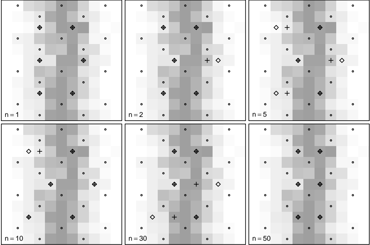
Figure 4: Approximate (+) and simulated (◇) designs as the sample size of the observed data ( n ) varies.
