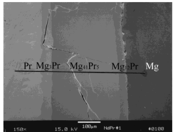
FIG. 6. SEM micrograph of the Mg–Pr diffusion couple taken across the diffusive interface. The trace of the EDS scan is shown.
