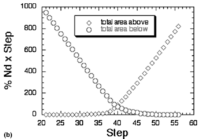
FIG. 8. (a) Close-up of the composition profile of Nd obtained from the SEM showing transition from pure Nd to MgNd, steps 21 to 56. (b) The determination of Boltzmann–Matano interface in Mg–Nd composition profile (see text).
