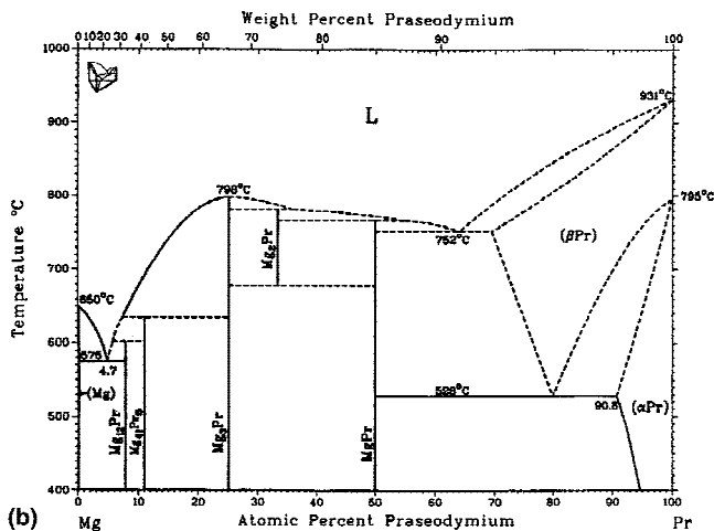
FIG. 7. (a) The Mg–Pr concentration profile obtained using EDS analysis. (b) Phase diagram of Mg–Pr (from Ref. 7).
