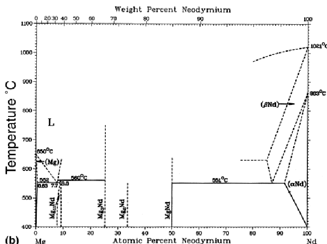
FIG. 3. (a) Mg–Nd concentration profile obtained using EDS analysis. (b) Phase diagram of Mg–Nd (from Ref. 7).
