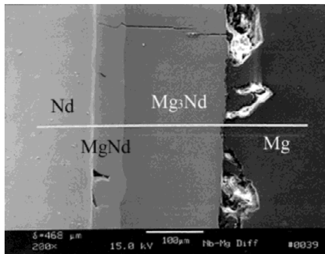
FIG. 2. SEM micrograph of the Mg–Nd diffusion couple taken across the diffusive interface. The trace of the EDS scan is shown.
