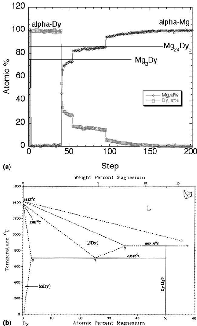
FIG. 5. (a) Mg–Dy concentration profile obtained using EDS analysis. (b) Phase diagram of Mg–Dy (from Ref. 7).
