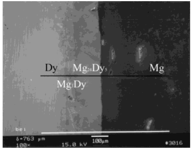
FIG. 4. SEM micrograph of the Mg–Dy diffusion couple taken across the diffusive interface. The trace of the EDS scan is shown.
