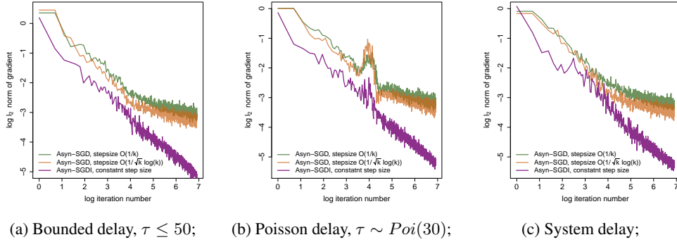
Figure 3: Simulation results for the convergence of Async-SGD and Async-SGDI with three kinds of delay on MLE for MVN covariance matrix.
