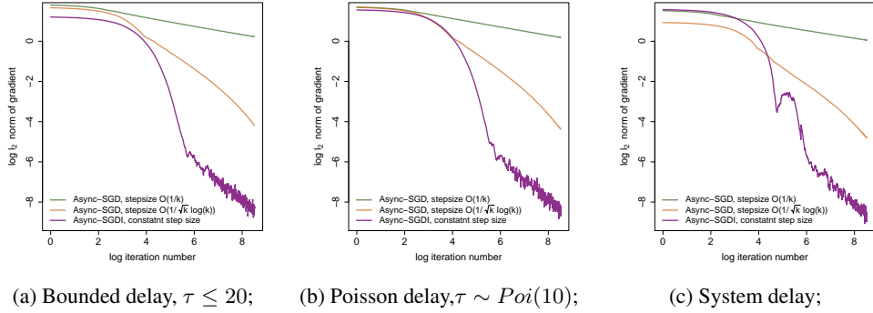
Figure 2: Simulation results for the convergence of Async-SGD and Async-SGDI with three kinds of delay on matrix completion problem.
