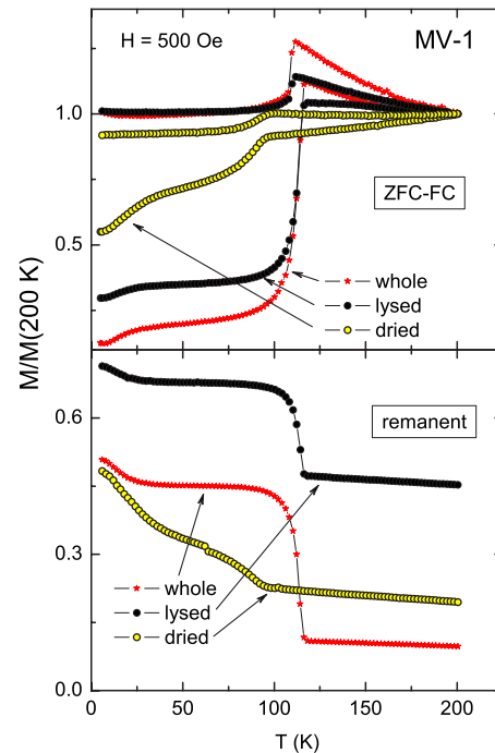
FIG. 4. (Color online) M(T) measurements from magnetite produced by cells of strain MV-1 with chains (whole and lysed cells) and dried cells with disrupted chains (individual particles). Top panel shows ZFC-W and FC-C measurements, whereas bottom panel shows Rem-W data.
