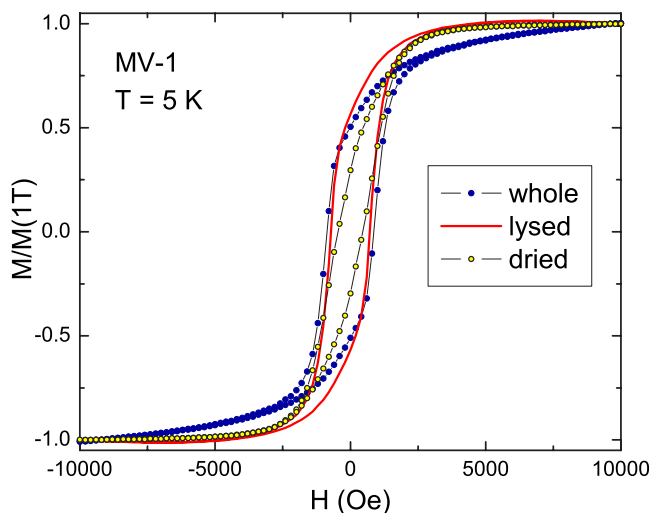
FIG. 7. (Color online) Comparison of the 5 K M(H) hysteresis loops from the whole, lysed, and freeze-dried cells from strain MV-1, which contain magnetite nanoparticles.
