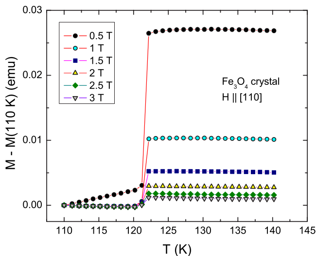
FIG. 3. (Color online) Magnetic signature of the Verwey transition in a \text{Fe}_3\text{O}_4 single crystal measured at different magnetic field strengths as indicated in the graph.
