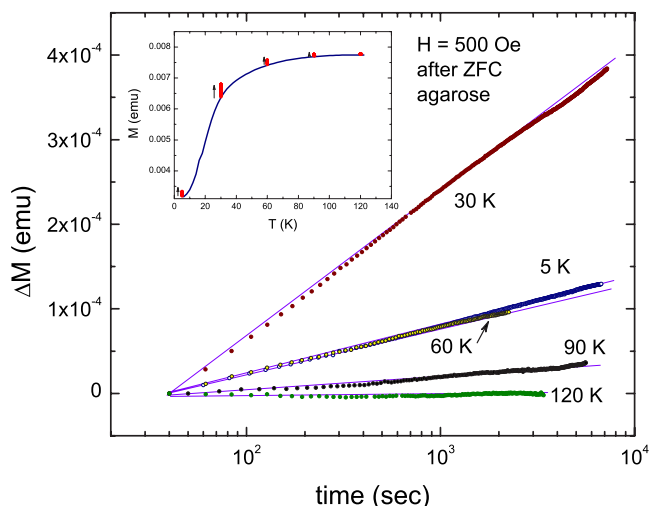
FIG. 8. (Color online) Magnetic relaxation in synthetic magnetite nanoparticles (in agarose) measured at H=500 Oe applied after ZFC to the indicated temperature. Inset shows the corresponding ZFC-W temperature scan.
