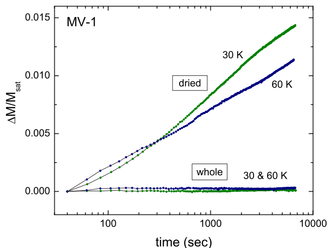
FIG. 9. (Color online) Magnetic relaxation curves measured in magnetite nanocrystals produced by strain MV-1 at H=500 Oe applied after ZFC. The two lower lines are for intact frozen bacterial cells, whereas the upper lines are for dried cells with disassembled chains.
