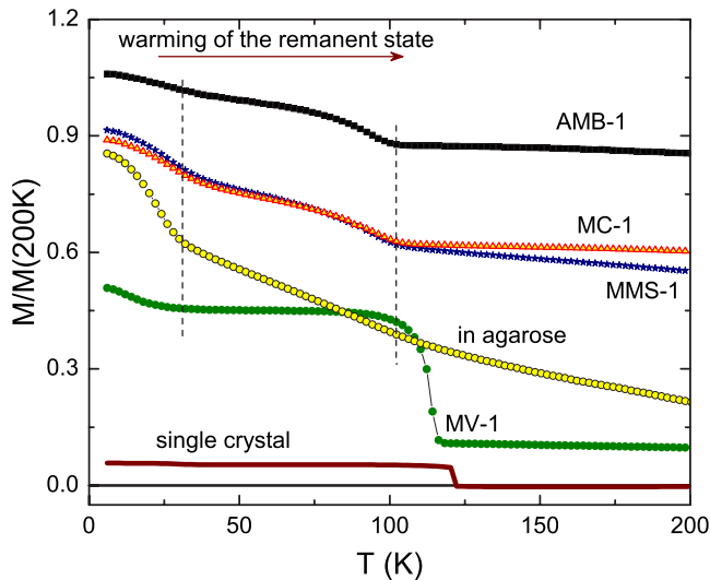
FIG. 2. (Color online) Annealing of the remanent state (Rem-W) in six different samples of magnetite as indicated by labels. Normalization at 200 K was done using values obtained from the ZFC-W curves at 500 Oe as described in the text.
