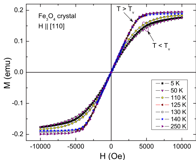
FIG. 6. (Color online) Magnetization loops measured at different temperatures in a single magnetite crystal along the [110] direction. No magnetic hysteresis is observed and there is likely a strong change in magnetic anisotropy at the Verwey transition.
