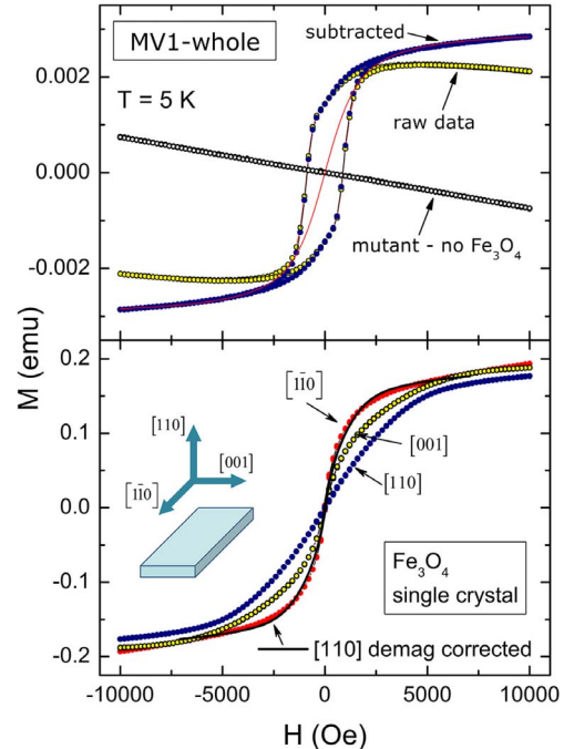
FIG. 5. (Color online) M(H) loops measured at 5 K in (top) frozen cell suspension of strain MV-1, whose magnetosomes contain \text{Fe}_3\text{O}_4 nanoparticles. The diamagnetic background from cells of a nonmagnetic mutant strain of MV-1 (contains no magnetite) can be subtracted from the wild-type magnetic strain. The solid curve (red online) is a fit to the Langevin function. (Bottom) Single crystal \text{Fe}_3\text{O}_4 and schematics of its geometry. See discussion in the text.
