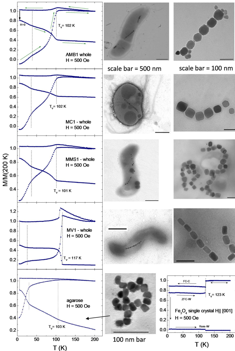
FIG. 1. (Color online) M(T) measurements of various forms of \text{Fe}_3\text{O}_4 nanoparticles. In each case, three measurements, shown here as three separate curves, were taken as described in the text—ZFC-W and FC-C at H=500 Oe, and then turning the field off and warming of the remanent magnetization. The top four rows correspond to biologically produced magnetite from four different whole bacterial cells—strains AMB-1, MC-1, MMS-1, and MV-1, respectively. For comparison, the lower left frame shows measurements of synthetic \text{Fe}_3\text{O}_4 nanoparticles and the lower right frame shows data from large single crystals. The middle column, except for the bottom figure, shows transmission electron micrographs (TEMs) of whole cells of the magnetotactic bacterial strains. The bottom image is a TEM of synthetic magnetite. The right column, except for the bottom figure, shows TEMs of magnetosome chains released from lysed cells.
