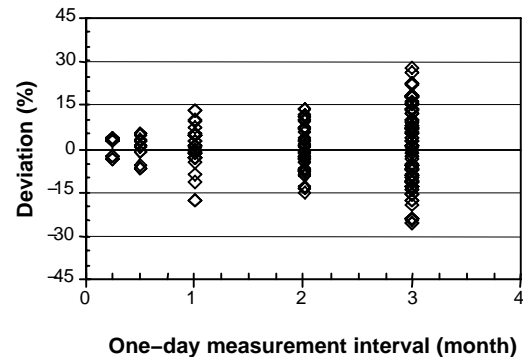
Figure 3. Relative deviation of ammonia emission rate based on the subsets of different one-day measurement intervals from the reference ER of the full dataset for four high-rise layer houses.
