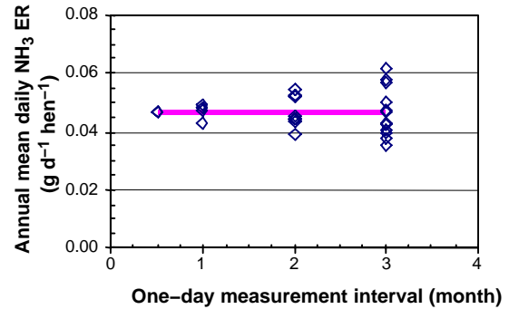
Figure 2. Annual mean daily ammonia emission rate (ER) from subsets at different one-day measurement intervals for a manure-belt layer house. Straight line represents the reference ER from the full dataset.
