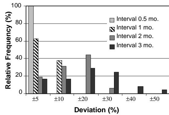
Figure 6. Frequency distributions of ammonia emission rate deviations from the reference value at different one-day measurement intervals for the manure belt houses.
