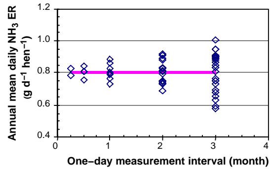
Figure 1. Annual mean daily ammonia emission rate (ER) from subsets at different one-day measurement intervals for a high-rise layer house. Straight line represents the reference ER from the full dataset.
