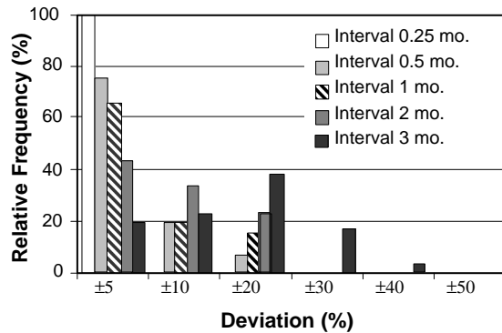
Figure 5. Frequency distributions of ammonia emission rate deviations from the reference value at different one-day measurement intervals for the high-rise layer houses.
