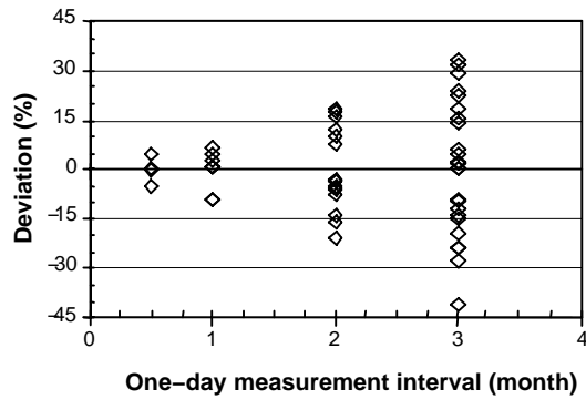
Figure 4. Relative deviation of ammonia emission rate based on the subsets of different one-day measurement intervals from the reference ER of the full dataset for two manure-belt houses.
