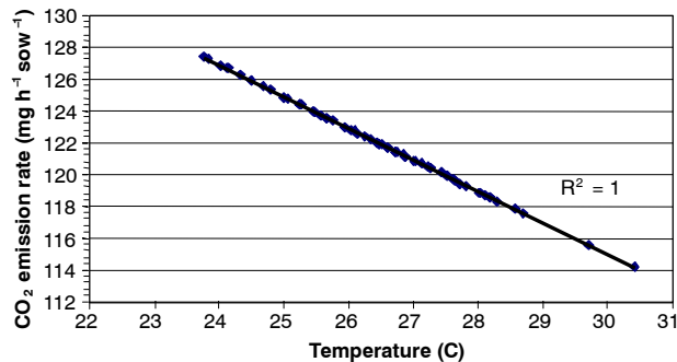
Figure 8. Carbon dioxide (CO 2 ) emission rate vs. inside temperature of the swine farrowing barn.
