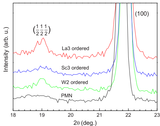
FIG. 2. (Color online) Partial x-ray diffraction spectra of La3-ordered, Sc3-ordered, and W2-ordered samples revealing the (1/2\ 1/2\ 1/2) superlattice peak at \sim 19^\circ . Data for PMN ceramics are included for reference.
