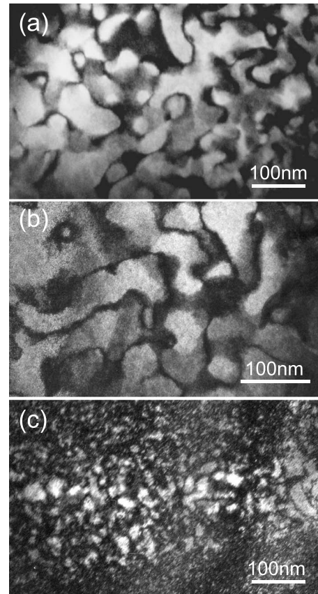
FIG. 3. TEM dark field micrographs of 1:1 cation-ordered domains formed with the (1/2\ 1/2\ 1/2) superlattice spot in the \langle 110 \rangle -zone axis selected area electron diffraction pattern. (a) La3 ordered, (b) Sc3 ordered, and (c) W2 ordered.
