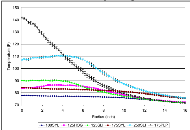
Figure 11a: Temperature and radial length comparison for metal fixture at 18-inch height (3 reps).
