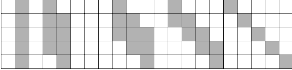
Figure 4: A shape sequence for Q_4 .
