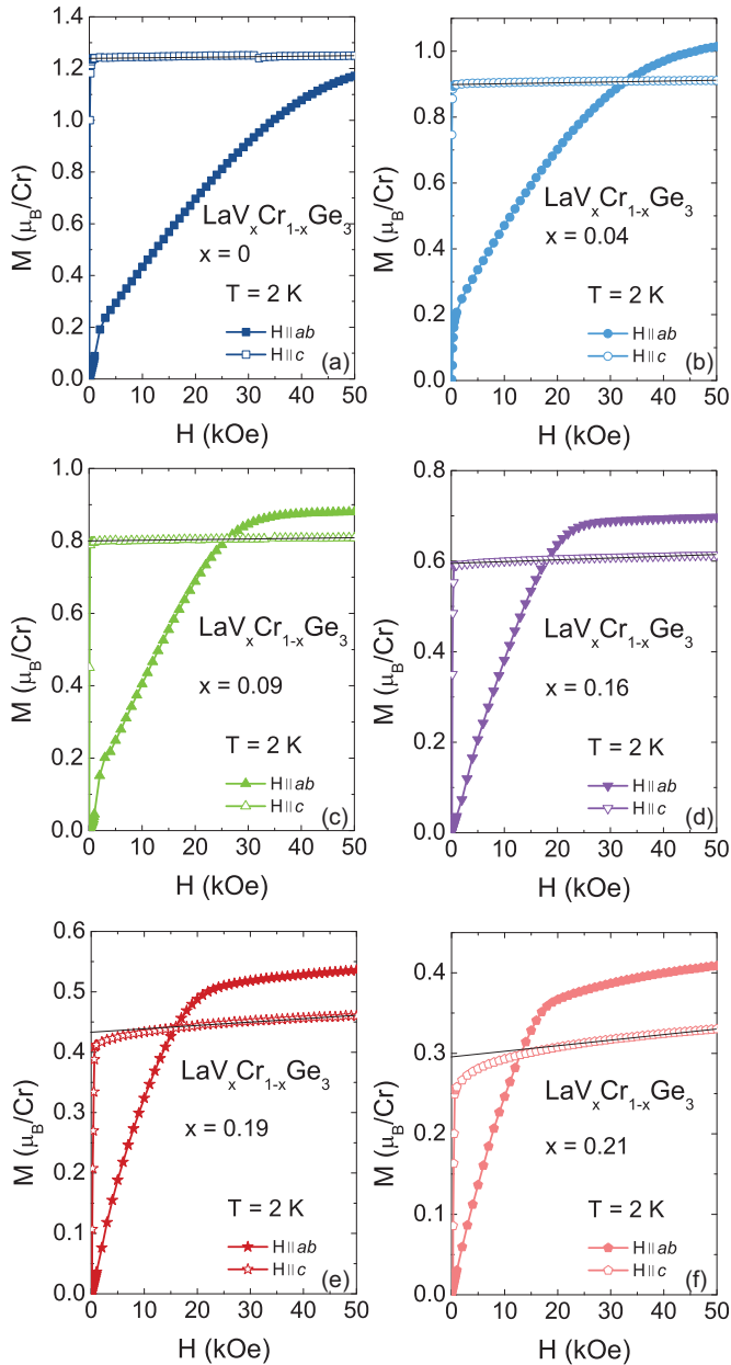
FIG. 3. (Color online) Anisotropic field-dependent magnetization data for \text{LaV}_x\text{Cr}_{1-x}\text{Ge}_3 ( x = 0–0.21 ) taken at 2 K. Fine solid lines through the high-field \mathbf{H} \parallel c data extrapolate back to H = 0 , \mu_S values shown in Table II.
