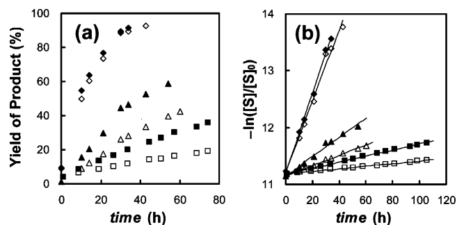
Figure 1. Methanolysis of diphenylmethyl chloride ( 2 ) with 20 mol % compound 1 in 5% ( \blacksquare ), 10% ( \blacktriangle ), and 15% ( \blacklozenge ) CD 3 OD/CCl 4 at 20 °C. The open data points ( \square , \triangle , \diamond ) are for the control experiments with no compound 1 present in the corresponding solvent mixtures. [S] is the concentration of the substrate at different times.
