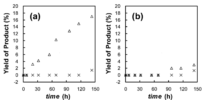
Figure 2. Competitive methanolysis of compounds 5 ( \Delta ) and 6 ( \times ) with (a) 20 mol % compound 1 and (b) without compound 1 in 5% \text{CD}_3\text{OD}/\text{CCl}_4 .
