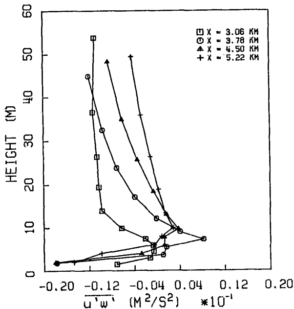
FIG. 7. Simulated Reynolds stress profiles at eight locations over Rattlesnake Mountain at 2300 PST 1 July 1980.
