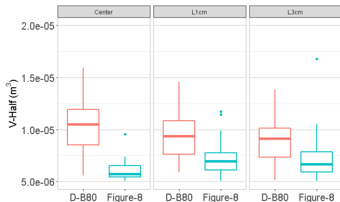
Fig. 9. Comparison of V-Half ( m^3 ) between two coils at each position
