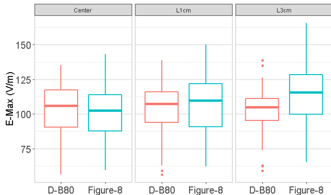
Fig. 8. Comparison of E-Max (V/m) between two coils at each position
