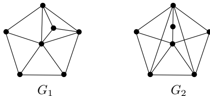
Figure 2.1: \mathcal{D}^L -cospectral graphs that have different degree and transmission sequences (see Example 2.1).
