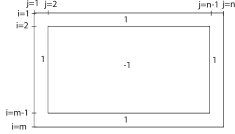
Figure 18: The diagram of zero and null spread for all vertices in P_m \boxtimes P_n , as established in Theorem 3.24. The vertices on the boundaries have n_v(P_m \boxtimes P_n) = z_v(P_m \boxtimes P_n) = 1 .
