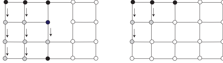
Figure 10: Diagrams for Observations 3.6 and 3.7
