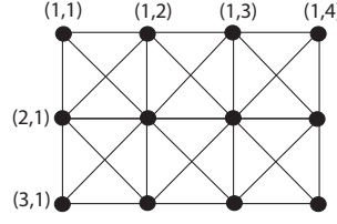
Figure 17: The 3 \times 4 strong product.
