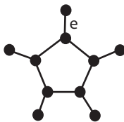
Figure 5: The pentasun H_5 for Example 2.18
