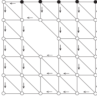
Figure 16: Optimal zero forcing set on a triangular grid graph minus a diagonal vertex.
