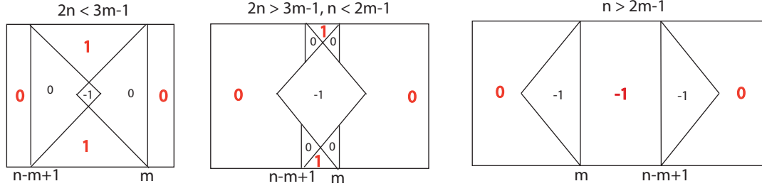
Figure 13: Schematic diagram of zero edge spreads for horizontal edges (parallel to the long side) in non-square grid graphs. Results established are in large type and those conjectured are small type.
