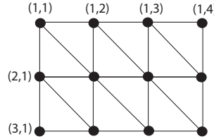
Figure 14: The 3 \times 4 triangular grid graph.
