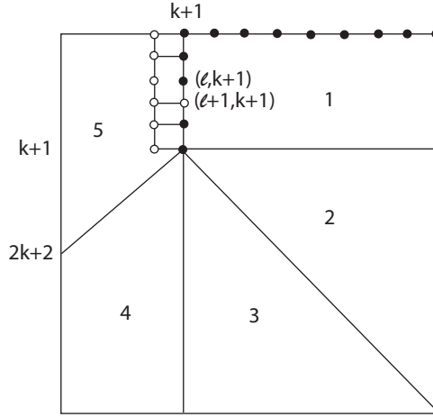
Figure 11: Diagram of Theorem 3.8
