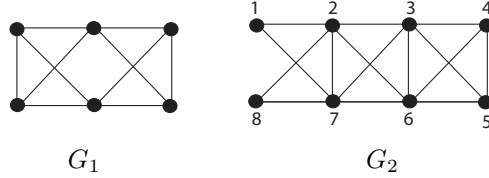
Figure 20: The graphs G_1 and G_2 for Lemma 3.26
