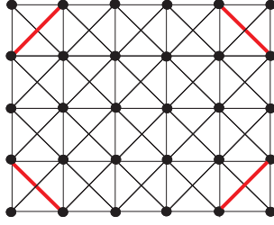
Figure 21: Zero edge spreads in the king grid P_m \boxtimes P_n, 4 \leq m \leq n . The four thick edges have n_e(P_m \boxtimes P_n) = z_e(P_m \boxtimes P_n) = 1 and all other edges have n_e(P_m \boxtimes P_n) = z_e(P_m \boxtimes P_n) = 0 .
