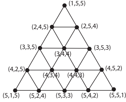
Figure 7: The supertriangle T_5
