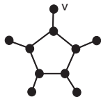
Figure 1: The pentasun H_5
