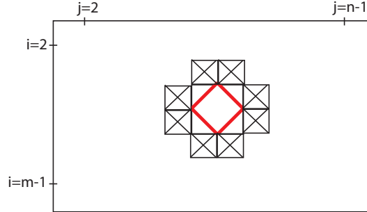
Figure 19: Covering of king grid for zero spread -1 .
