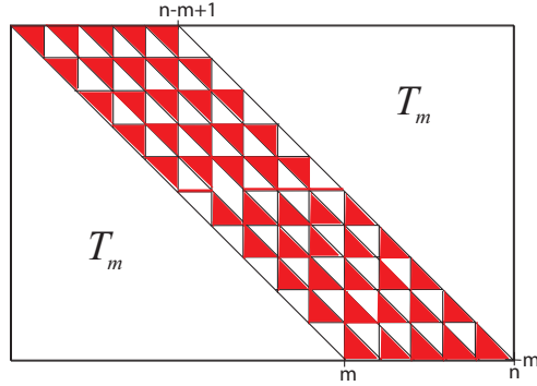
Figure 15: A covering of the edges of the subgraph H - e in a triangular grid graph, assuming the two large supertriangles are covered.
