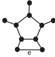
Figure 6: Graph G for Example 2.19
