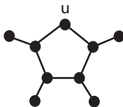
Figure 3: A counterexample to the converse of Theorem 2.8
