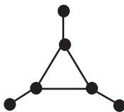
Figure 4: The graph H_3 in Example 2.11
