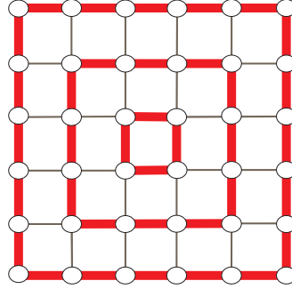
Figure 12: Schematic diagram of bull's-eye theorem and conjecture: The thick lines (concentric squares) have edge spread 1. The thin lines have edge spread 0 for the grid graph P_6 \square P_6 that is shown, and are conjectured to have edge spread 0 for all square grid graphs.
