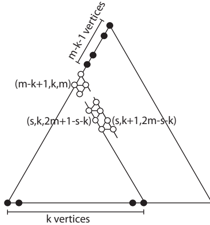
Figure 8: Diagram for Theorem 3.1.
