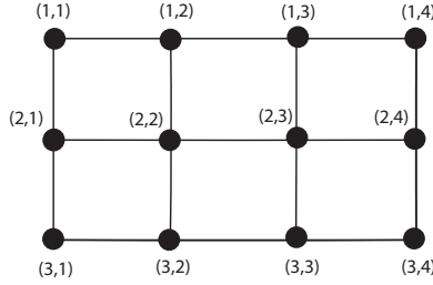
Figure 9: The 3 \times 4 grid graph P_3 \square P_4 .
