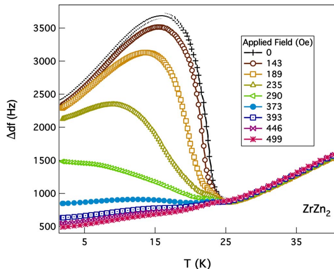
FIG. 2. (Color online) Change in dynamic susceptibility of a single crystal of \text{ZrZn}_2 in various applied fields.
