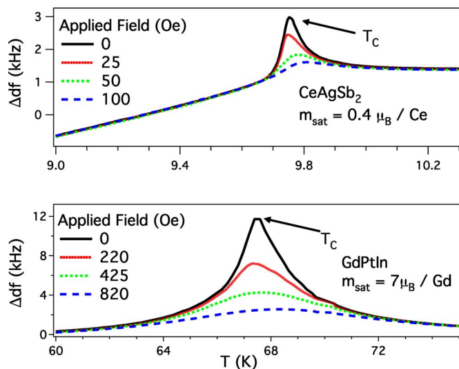
FIG. 4. (Color online) Comparison of the zero field resonator response to the small moment \text{CeAgSb}_2 (top) with the large moment \text{GdPtIn} (bottom), both LFM compounds.
