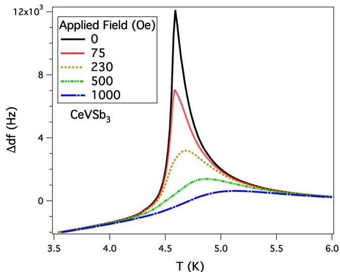
FIG. 1. (Color online) Frequency shift ( \propto \chi ) of TDR resonance in single crystal \text{CeVSb}_3 . The sharp peak is at T_C \approx 4.5 K.
