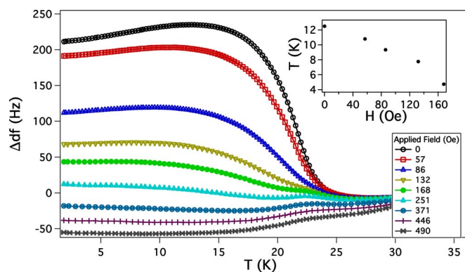
FIG. 3. (Color online) Response of TDR to \text{ZrZn}_2 powder in epoxy. Inset: Scatter plot of temperature of maximum vs applied field.
