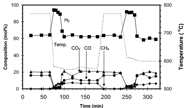
Figure 3. Product gas composition ( \text{H}_2\text{O} and \text{C}_7\text{H}_8 free) produced by reacting steam with \text{CO} , \text{CH}_4 , and \text{C}_7\text{H}_8 using 3 mol of \text{H}_2\text{O}/\text{mol} of \text{C} at 1.0 atm.
